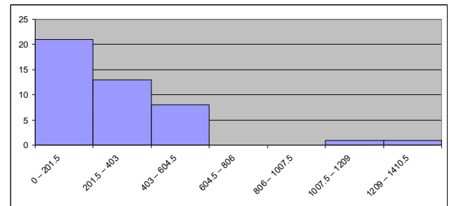
Figure 1. The graph of the histogram of the climate-weather change process conditional sojourn time C_{12}
