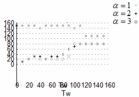
Figure 13. Optimal value of T for various failure intensity of the component B: R_B = \exp(-(t/100))^\alpha .
