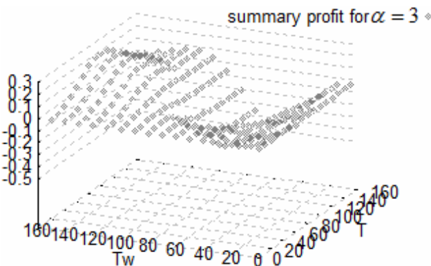
Figure 16. Summary profit resulting from reusing of elements B in new production for R_B = \exp(-(t/100))^3 .
