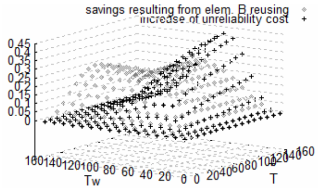
Figure 7. Increase of unreliability costs and savings resulting from the reusing policy according to Eqn12 with maximal possible number of reusable returns.
