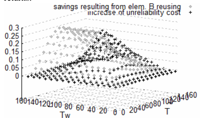
Figure 8. Increase of unreliability costs and savings resulting from the reusing policy according to Eqn12 with minimal possible number of reusable returns.
